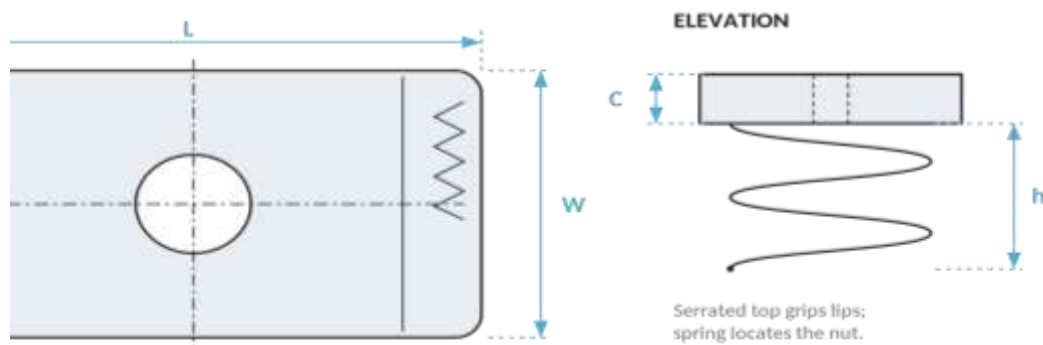
Short spring channel nut — plan and elevation, dimensions not to scale
