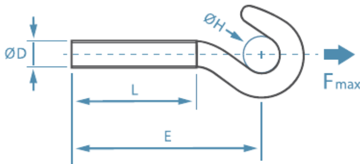
Hook bolt technical drawing. Not to scale.
