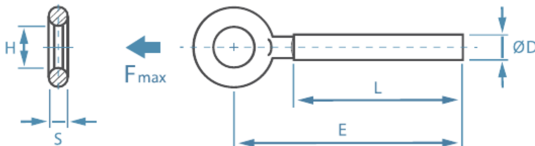
Eyebolt technical drawing. Not to scale.
