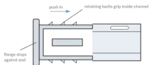
SECTION (PLUGS IN)
