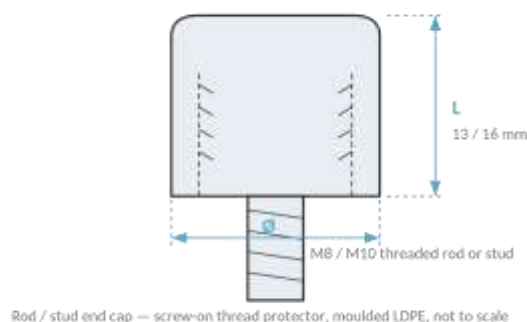
Rod / stud end cap — screw-on thread protector, moulded LDPE, not to scale
