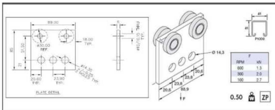
Technical drawing - P2950 double wheel channel trolley assembly. Dimensions in mm.
