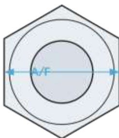
Hexagon head with domed (closed) crown
