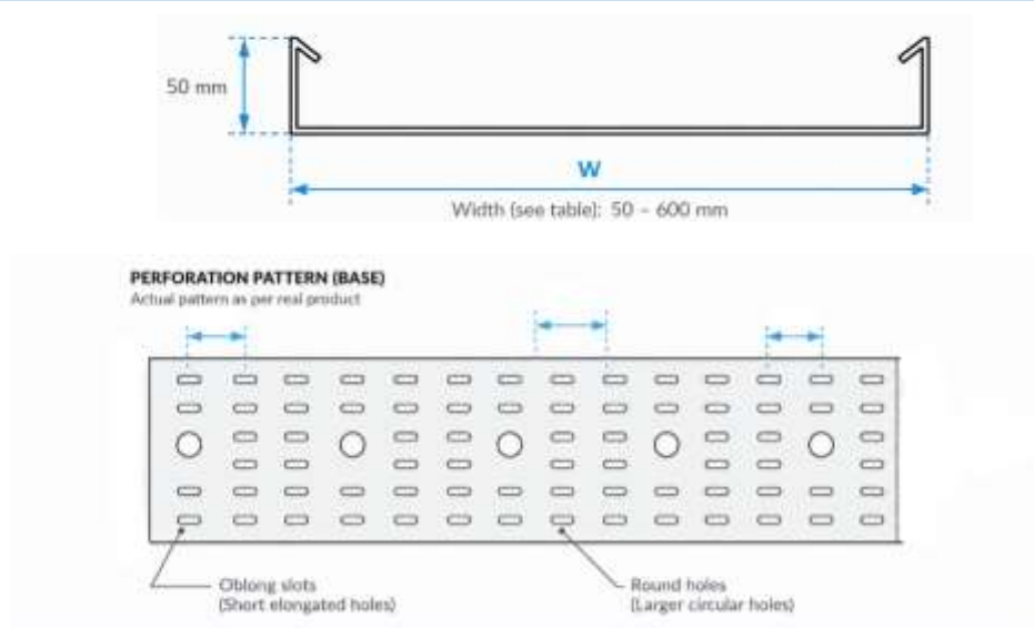
Heavy Duty Cable Tray — cross-section and base detail, dimensions in mm, not to scale
