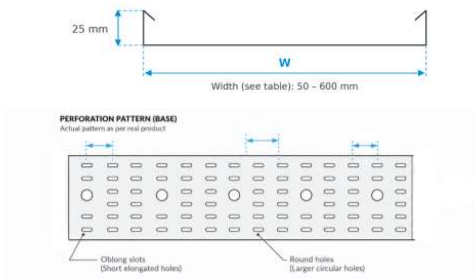
Medium Duty Cable Tray — cross-section and base detail, dimensions in mm, not to scale
