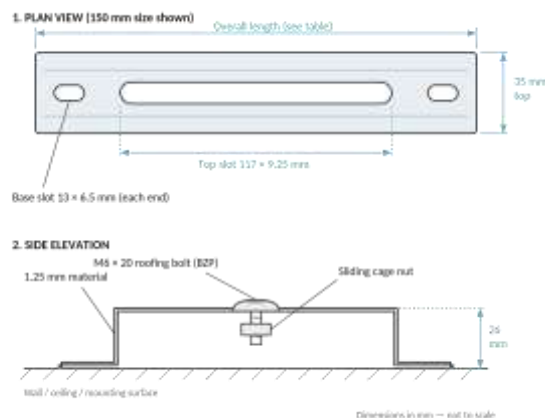
Representative stand off bracket (150 mm size) — dimensions in mm, not to scale
