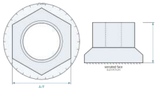
Hex serrated flange nut — plan and elevation, dimensions not to scale
