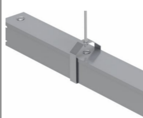
Threaded Rod Hanger for 50mm Cable Trunking
