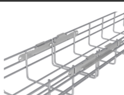
Straight Fast Click Connector – Stainless Steel (A2)
