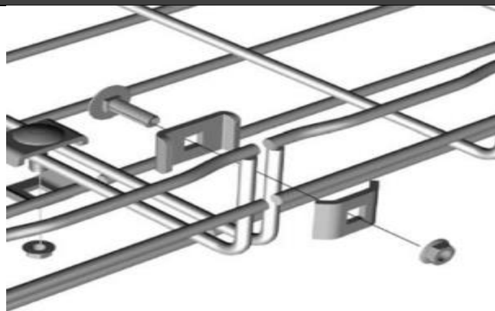
Reinforced Joint Clamp / Connector
